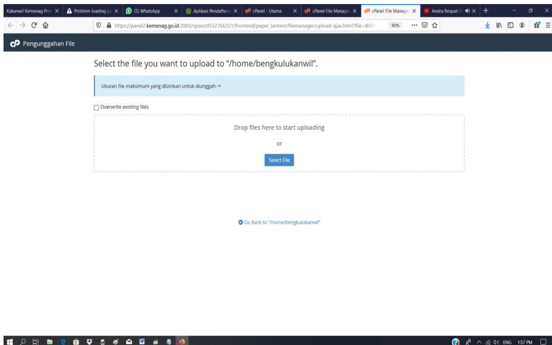
Proses Upload
