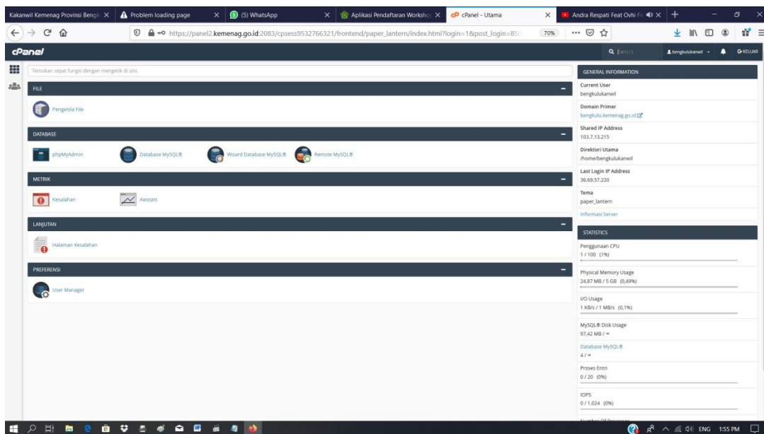
Dasboard Cpanel
